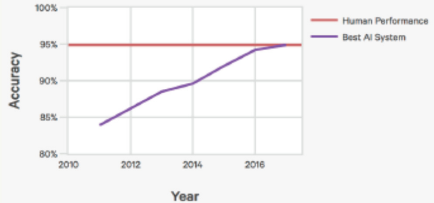
Speech Recognition, Switchboard HUB5'00
