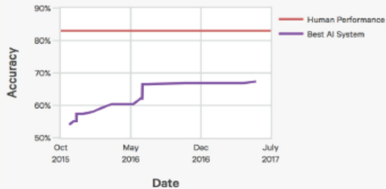
Visual Question Answering, VQA 1.0
